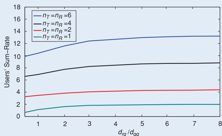
[FIG6] Sum rate of the users versus the inter-pair distance d_{rq}/d_{qq} ; d_{rq} = d_{qr} , d_{rr} = d_{qq} = 1 , \forall r, q , for different numbers of transmit/receive antennas.
