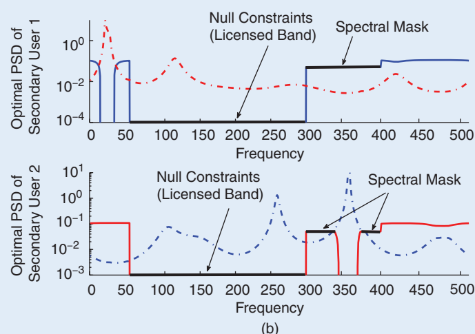
[FIG5] Spectrum sharing among one primary user [subplot (a)] and two secondary users [subplot (b)]: Optimal PSD of each link (solid lines), and PSD of the MUI-plus-thermal noise normalized by the channel transfer function square modulus of the link (dashed-dot line).
